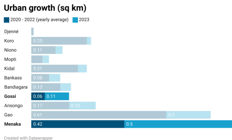
Figure 19: Urban growth in 2020 – 2023 for locations of interest in Mali.
